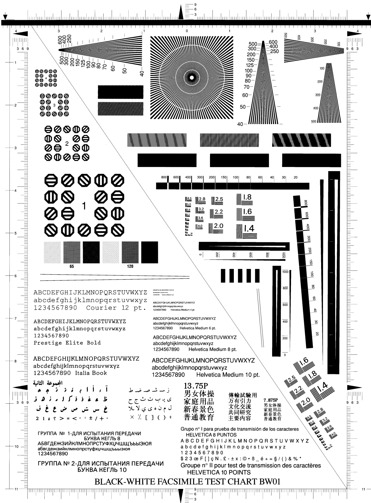
Figure 9/T.24 – Test Pattern Facsimile Test Chart BW01
